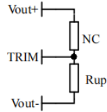
Voltage up regulation: add resistor R_{up} between Trim and output negative R_{up} = 6.375 / \Delta U - 5.1 (K \Omega )
