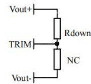
Voltage Down: Add resistor R_{down} between Trim and output positive R_{down} = 36 * (24 - 2.5 - \Delta U) / \Delta U - 5.1 (K \Omega )
