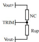
Voltage up regulation: add resistor R_{up} between Trim and output negative R_{up} = 90 / \Delta U - 5.1 (K \Omega )
