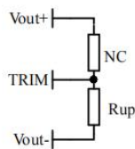
Voltage up regulation: add resistor R_{up} between Trim and output negative R_{up} = 140 / \Delta U - 5.1 (K \Omega )
