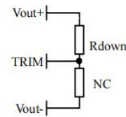
Voltage Down: Add resistor R_{down} between Trim and output positive R_{down} = 56 * (48 - 2.5 - \Delta U) / \Delta U - 5.1 (K \Omega )
